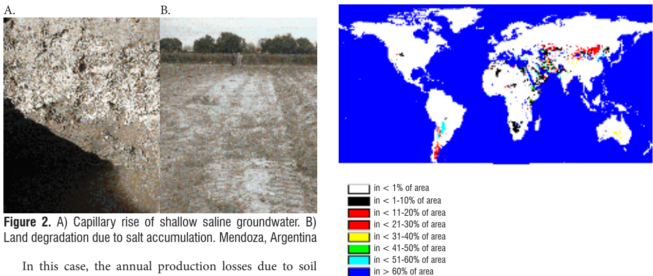
Figure 3. The world map of saline soils (FAO/UNESCO 2003)
